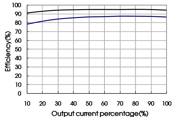
Positive output efficiency Vs output load (Vin=Vin-nominal)
